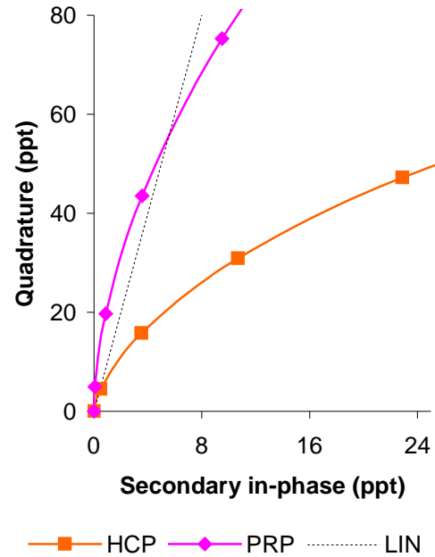
Figure 2: DUALEM arrays and LIN.
